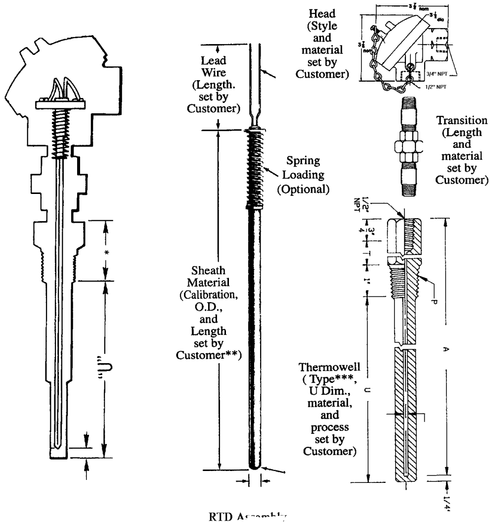
RTD Assembly
